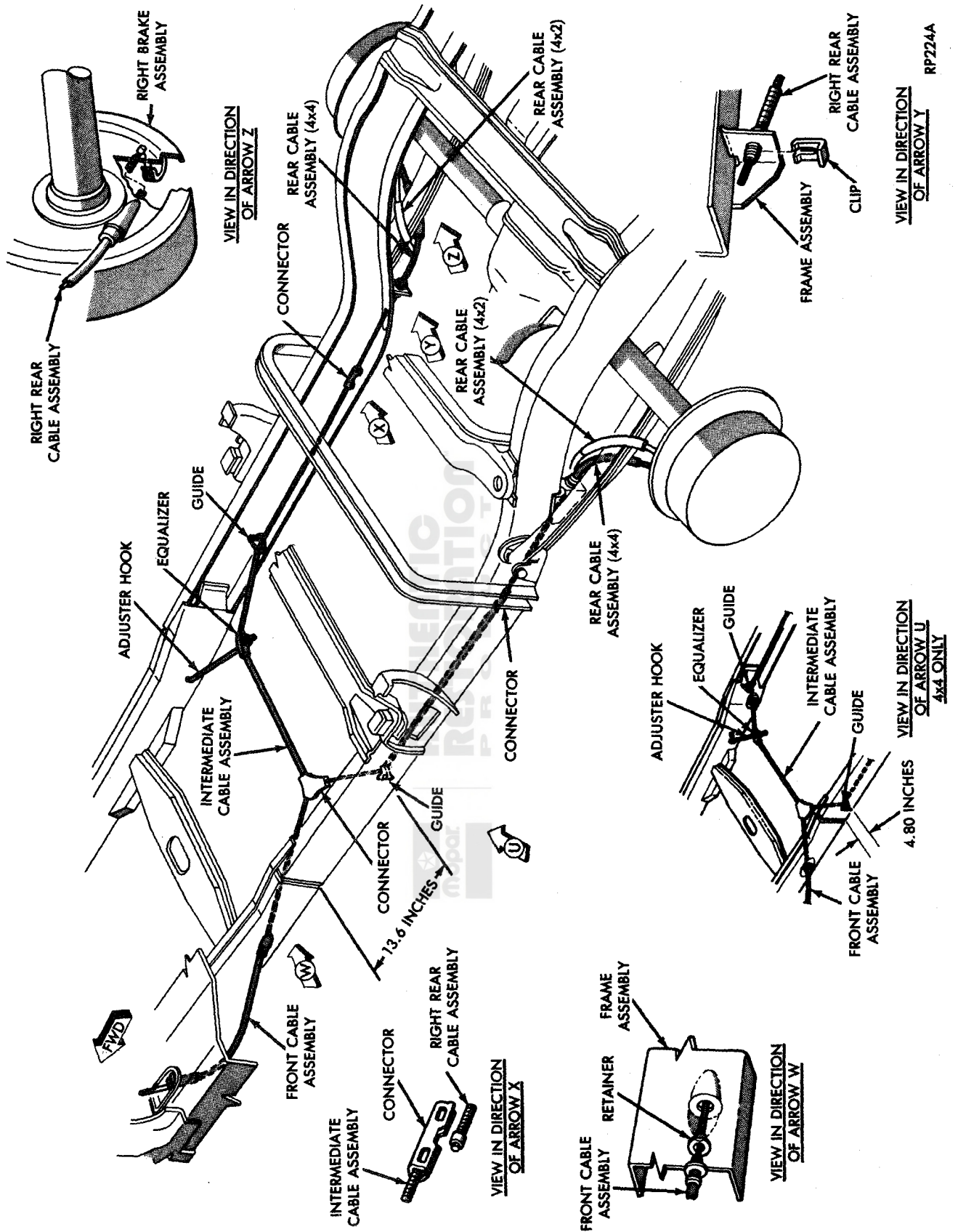
Fig. 1—Parking Brake Cable Routing
