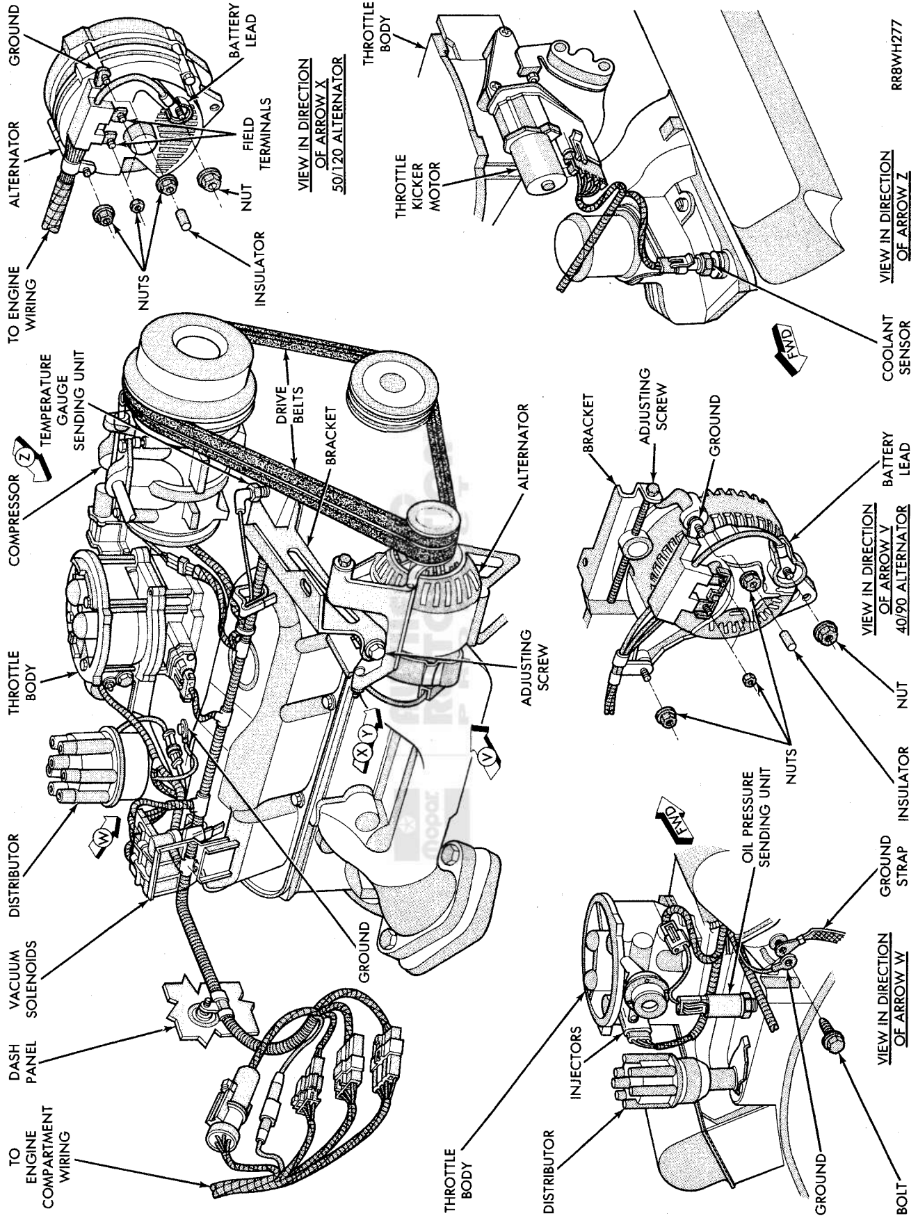
Fig. 21—Engine Wiring and Component Identification 3.9L Engine
