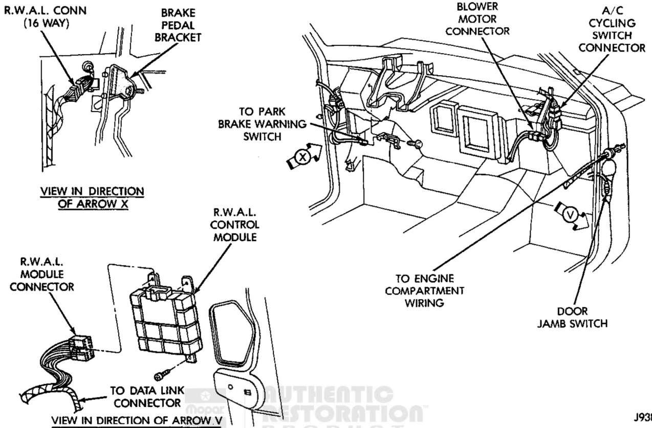
Fig. 6 Instrument Panel Wiring
