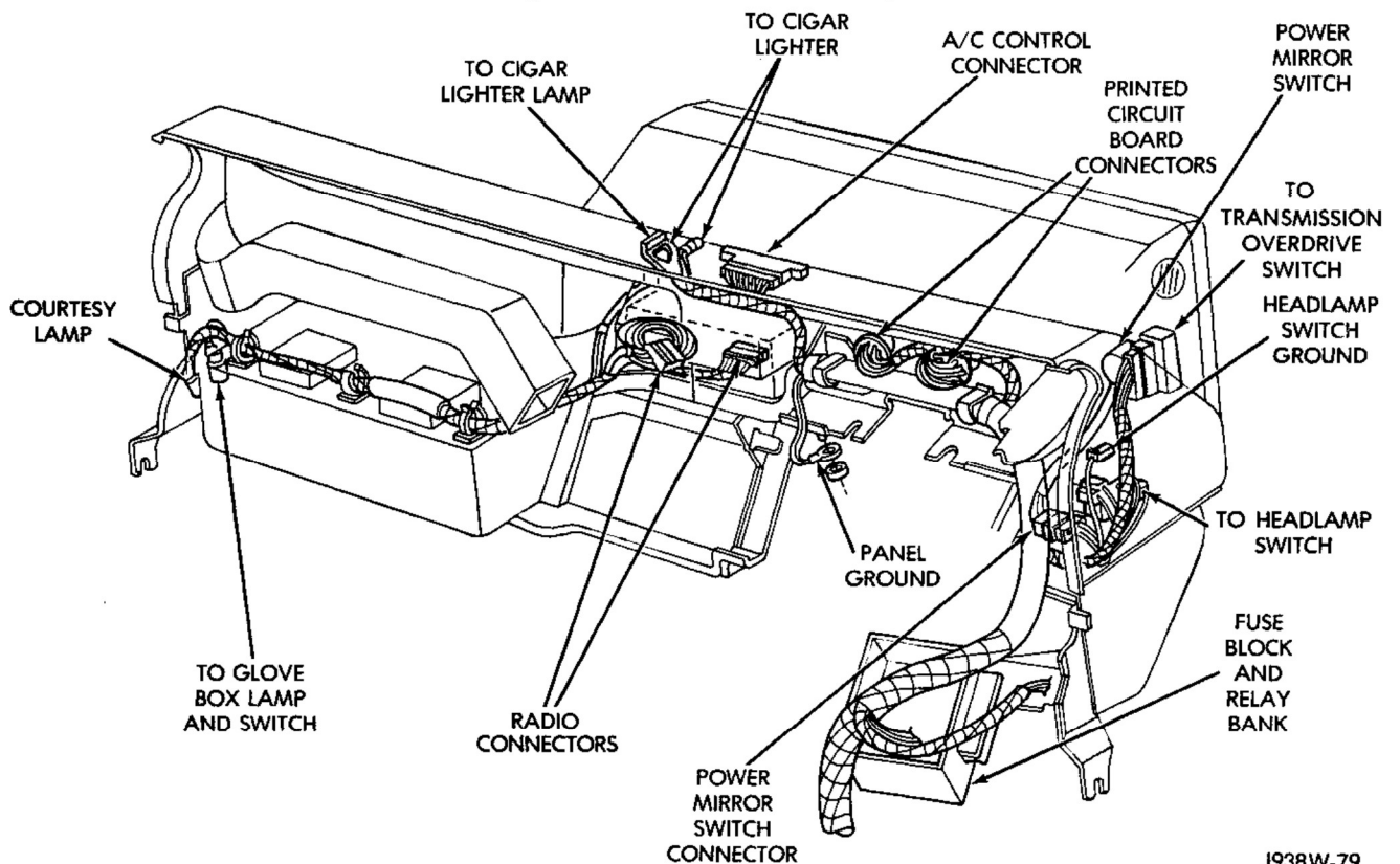
Fig. 7 Instrument Panel Wiring (Connections)
