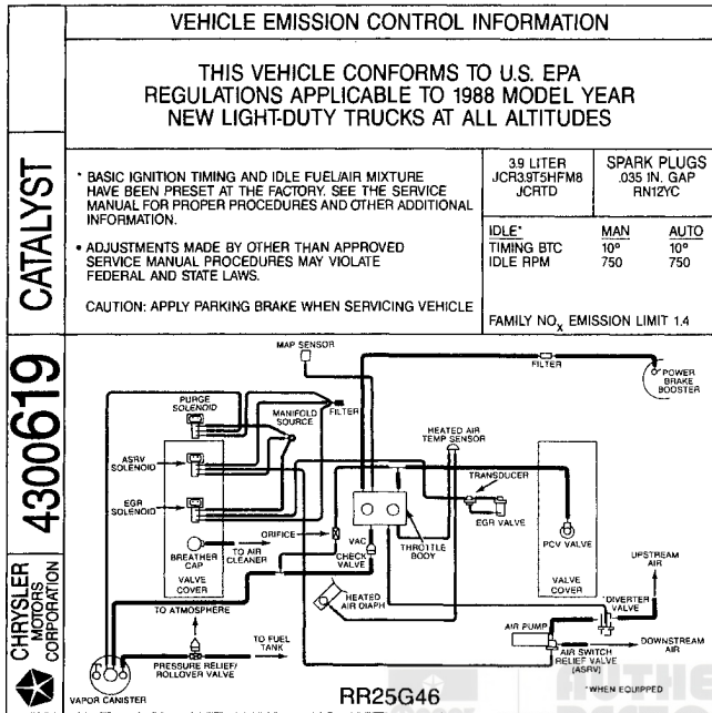
Fig. 9—Hose Routing Label 3.9L Federal and Altitude Fuel Injected Engines
