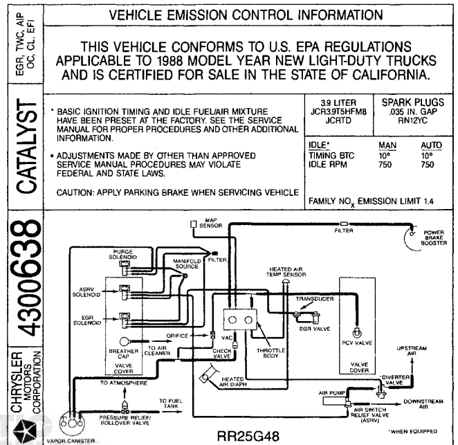
Fig. 11—Hose Routing Label 3.9L California Light Duty Fuel Injected Engines
