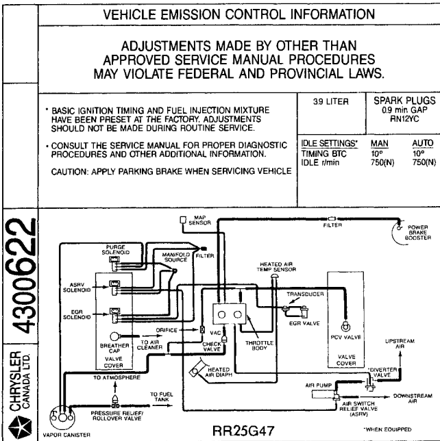
Fig. 10—Hose Routing Label 3.9L Canadian Fuel Injected Engines
