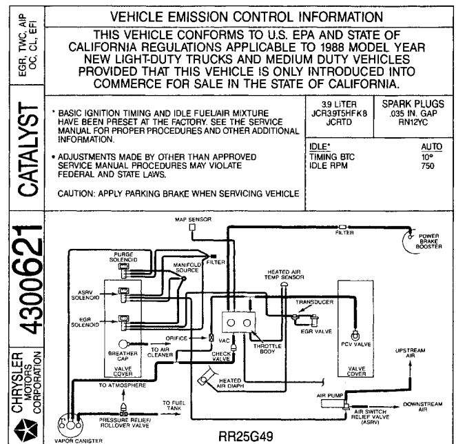
Fig. 12—Hose Routing Label 3.9L California Fuel Injected Engines
