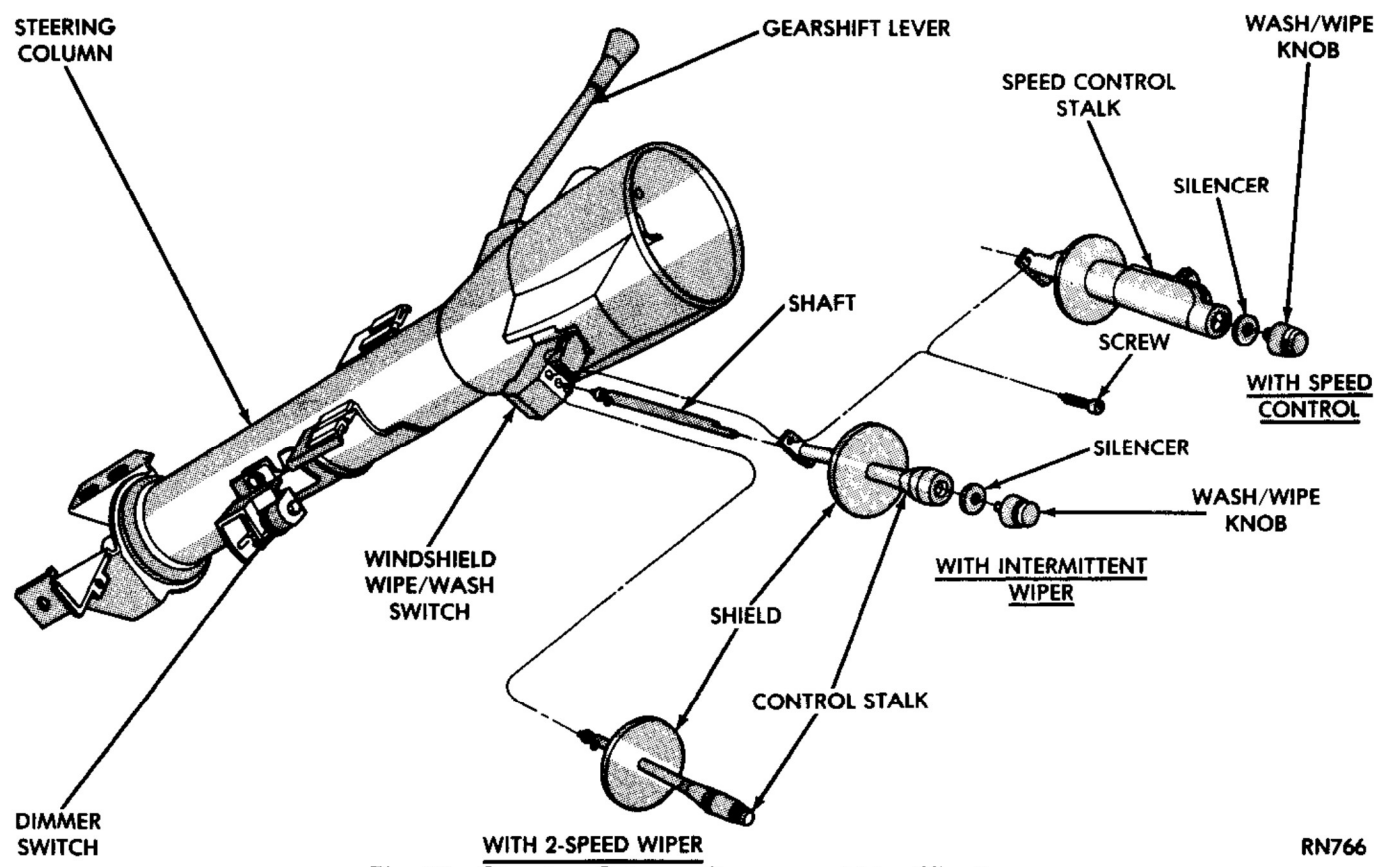
Fig. 10—Steering Column Component Identification
