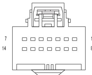
MODULE-TOTALLY INTEGRATED POWER C2
